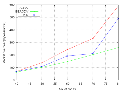
Fig. 3 Packet overhead of nodes
