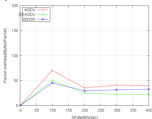
Fig. 4 Packet overhead during data sending
